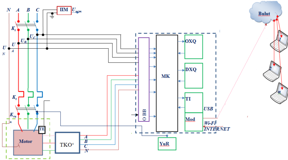
Fig. 1 – Structural diagram of the electrical energy monitoring system
