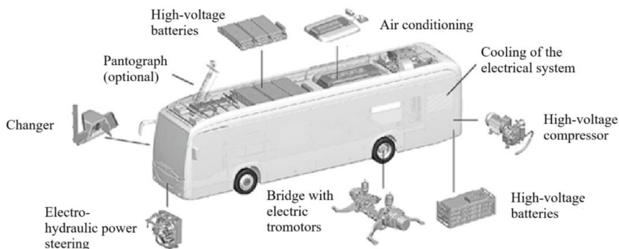
Fig. 2 – Electric bus structure
